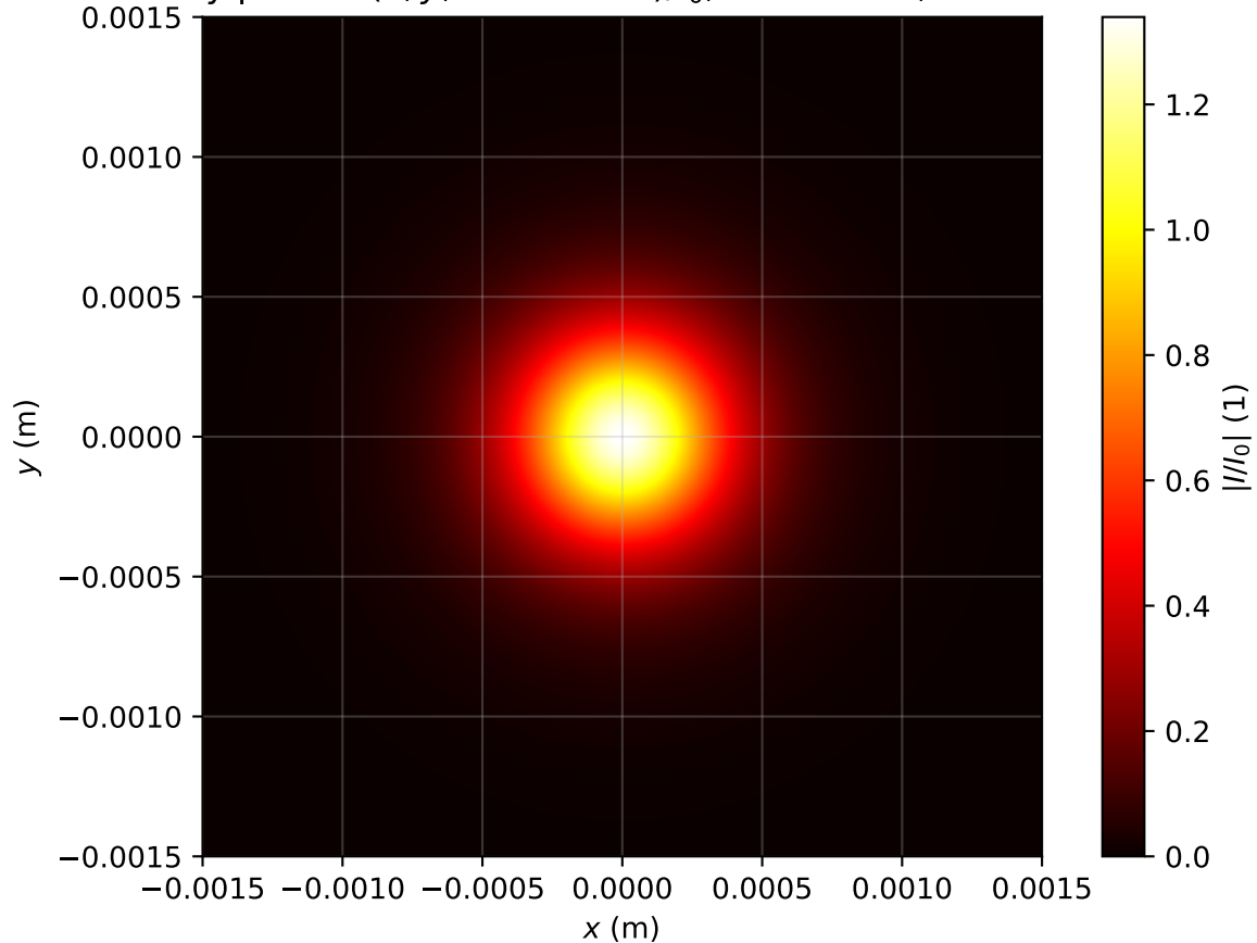
Intensity profile I(x, y, z = 1.831m)/I_0 , P_{in}=0.8P_{cr} , artificial time
